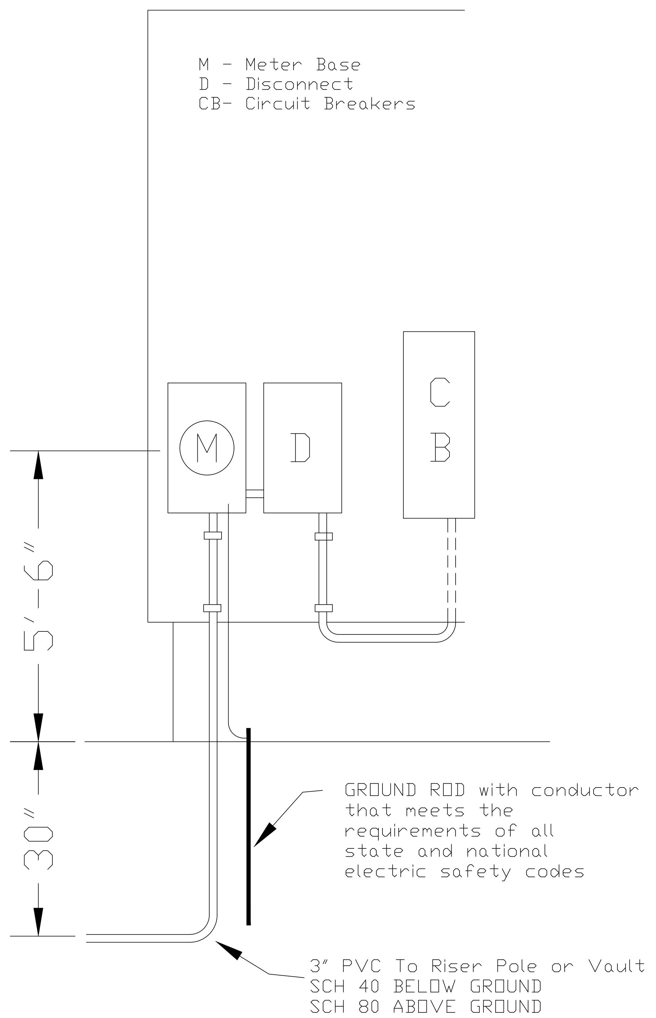
UNDERGROUND SERVICE TO MOBILE HOME
